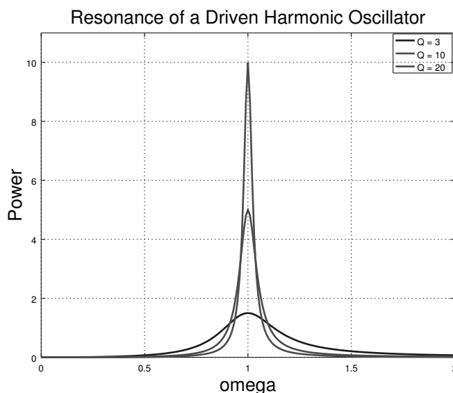
Figure 129: This plots the average power P(\omega) for three resonances. In these figures, F_0 = 1 , k = 1 , m = 1 (so \omega_0 = 1 ) and hence b is the only variable. Since Q = \omega_0/\Delta = m\omega_0/b we plot Q = 3, 10, 20 by selecting b = 0.333, 0.1, 0.05 . Thus P_{\max} = F_0^2/2b = 3/2, 5, 10 respectively (all in suitable units for the quantities involved). Note that the full width of e.g. the Q = 20 curve (with the sharpest/highest peak) is \sim 1/20 at P = P_{\max}/2 = 5 . P is the average power added to the oscillator by the driving force, which in turn in steady state motion must equal the average power lost to dissipative drag forces.
