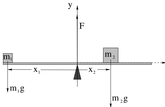
Figure 93: You are given m_1 , x_1 , and x_2 and are asked to find m_2 and F such that the see-saw is in static equilibrium .
