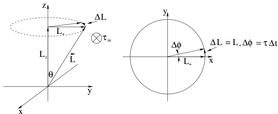
Figure 92: The cone swept out by the precession of the angular momentum vector, \vec{L} , as well as an “overhead view” of the trajectory of \vec{L}_{\perp} , the component of \vec{L} perpendicular to the z -axis.
