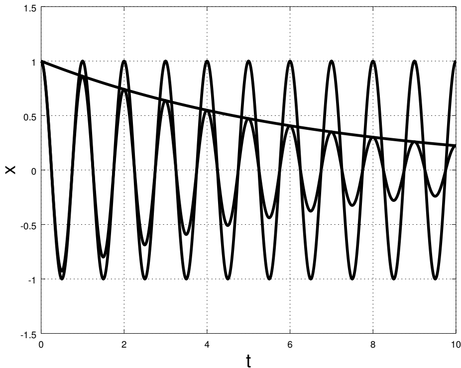
Figure 126: Two identical oscillators, one undamped (with \omega_0 = 2\pi , or if you prefer with an undamped period T_0 = 1 ) and one weakly damped ( b/m = 0.3 ).
