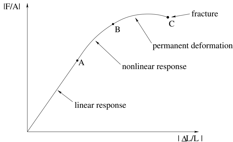
Figure 133: The slope of the linear response part of the curve is Young’s Modulus (note well the absolute magnitude signs). A marks the point where nonlinear response is first apparent. B marks the boundary where dislocations occur and permanent deformation of the material begins. C marks the point where there is a chain reaction – each defect produced produces on average at least one more defect at the same stress, so that the material “instantly” fractures.
