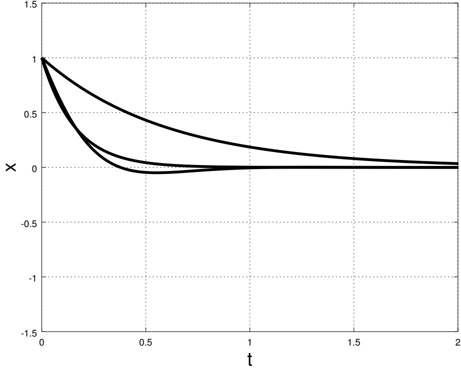
Figure 127: Three curves: Underdamped ( b/m = 2\pi ) barely oscillates. T' is now clearly longer than T_0 . Critically damped ( b/m = 4\pi ) goes exponentially to zero in minimum time. Overdamped ( b/m = 8\pi ) goes to zero exponentiall, but much more slowly.
